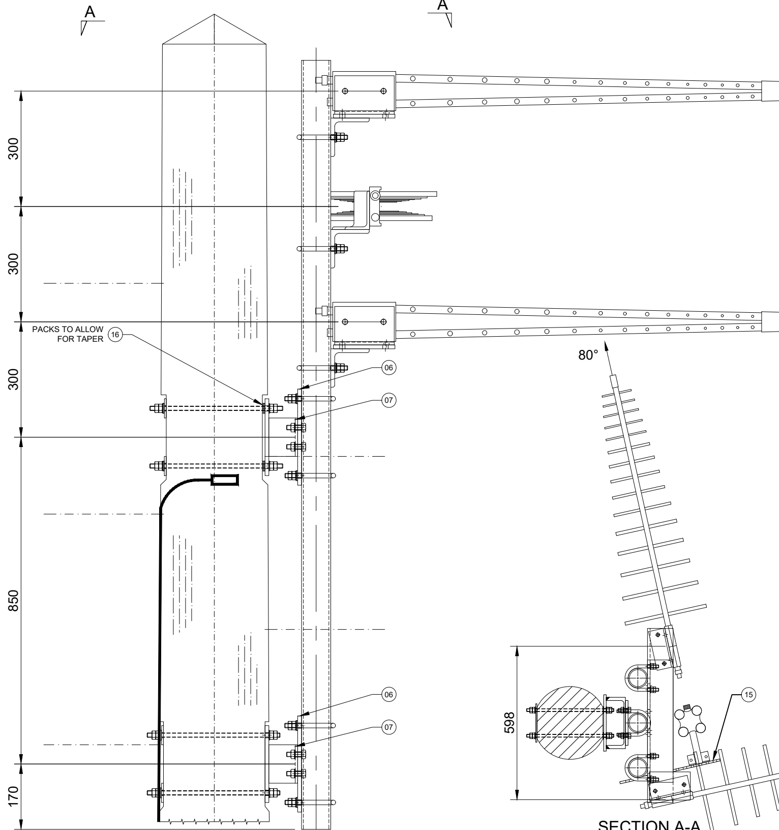
DETAIL G - Tx ANTENNA MOUNT Scale 1:10
