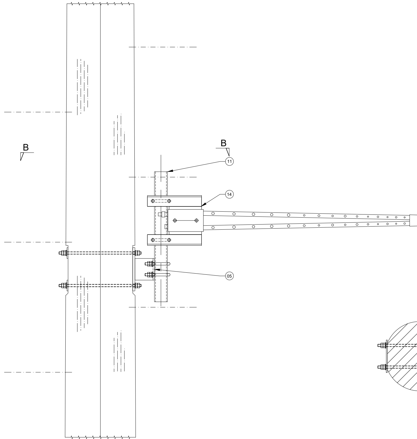
DETAIL H - Rx ANTENNA MOUNT Scale 1:10
