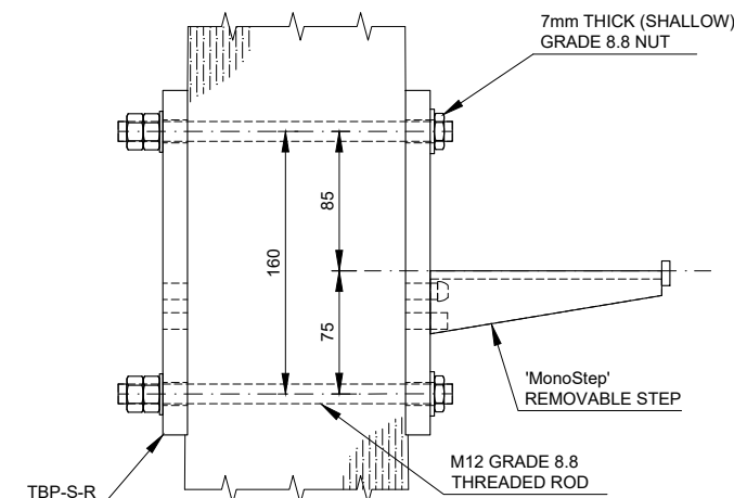
DETAIL F - REMOVABLE CLIMBING STEPS Scale 1:5
